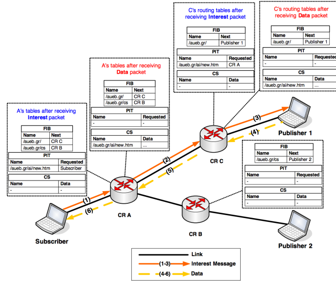
Figure 2.4.: Content centric networking architecture and flow. Adopted from [Xyl+14].
