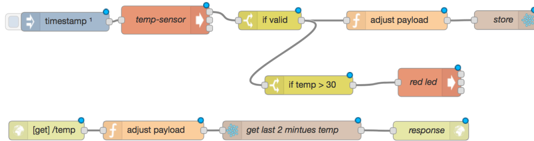
Figure 5.5.: A flow that reads temperature, stores it and starts a red LED if the temperature is above 30 degree Celsius.
