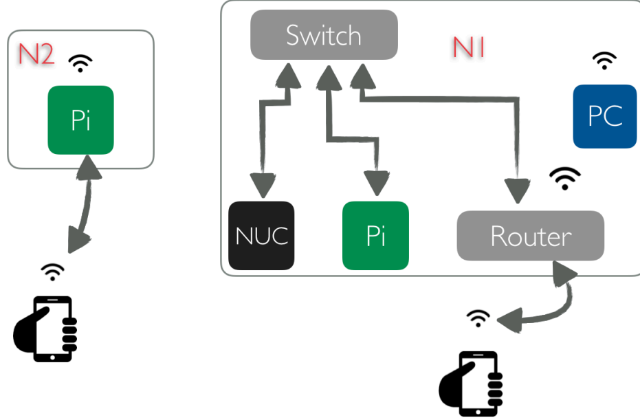
Figure 6.6.: Testbed setup for challenged and delay tolerant networks.
