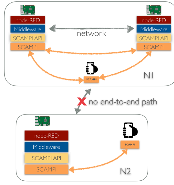
Figure 4.2.: SCAMPI synchronization even without an end-to-end path.
