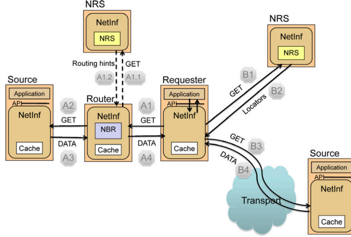
Figure 2.5.: NetInf routing flow example. Adopted from [Dan+13].
