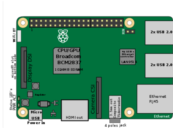
Figure 2.6.: Raspberry Pi 3 model B design. Adopted from [EFA].
