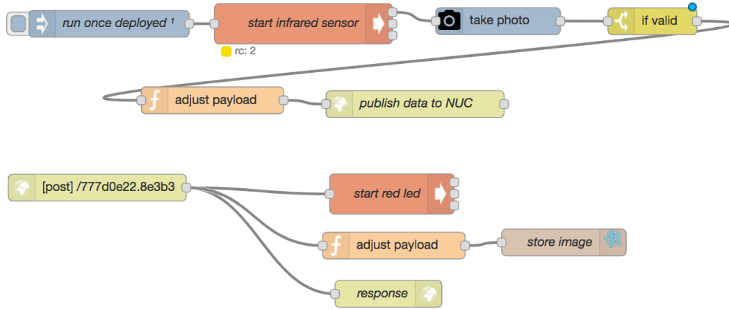
Figure 5.6.: A flow that detects motion, takes an image then publishes a message and stores incoming responses.
