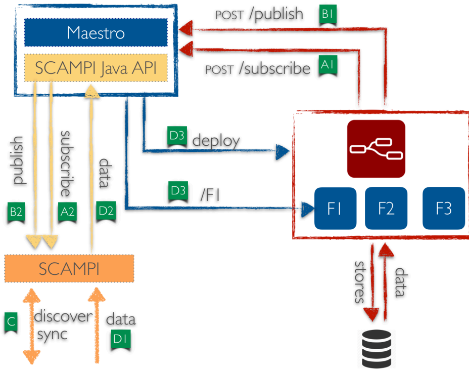
Figure 4.7.: Software framework architecture design.
