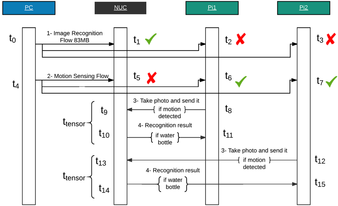
Figure 6.3.: Sequence diagram for recognizing water bottles.
