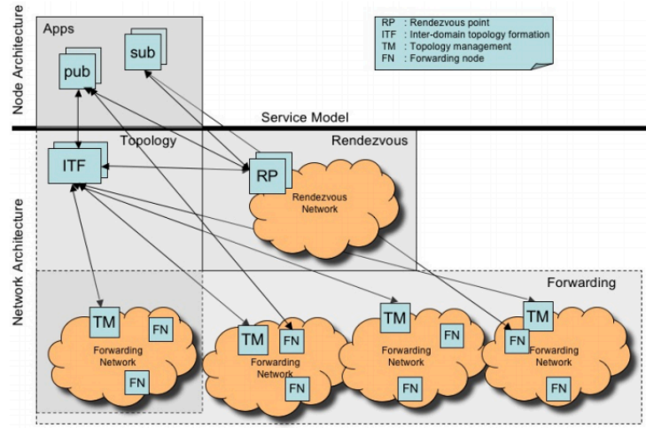
Figure 2.2.: ICN architecture by Dirk Trossen et al. Adopted from [TSS10].
