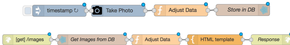
Figure 3.7.: Two separate computational flows describing the local IO composability through a database.
