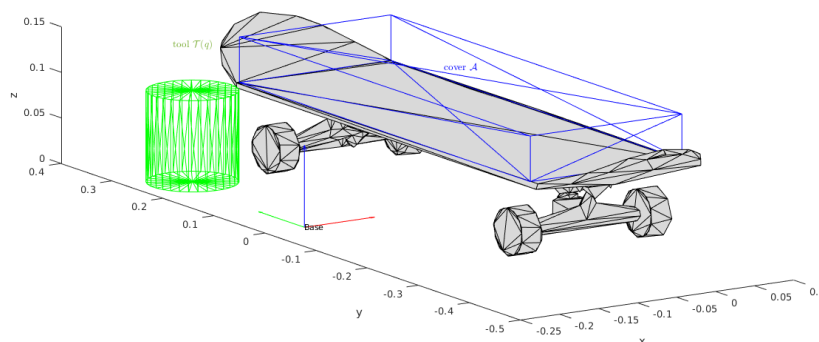
Finishing the surface of a skateboard with a cylindrical mill as a possible cover task.
